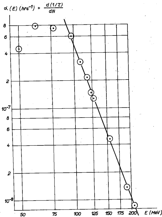
FIG. 2. Plot of the rate \alpha(E) , as defined in Eq. (1) of the text, versus the energy of electrons in a beam.
